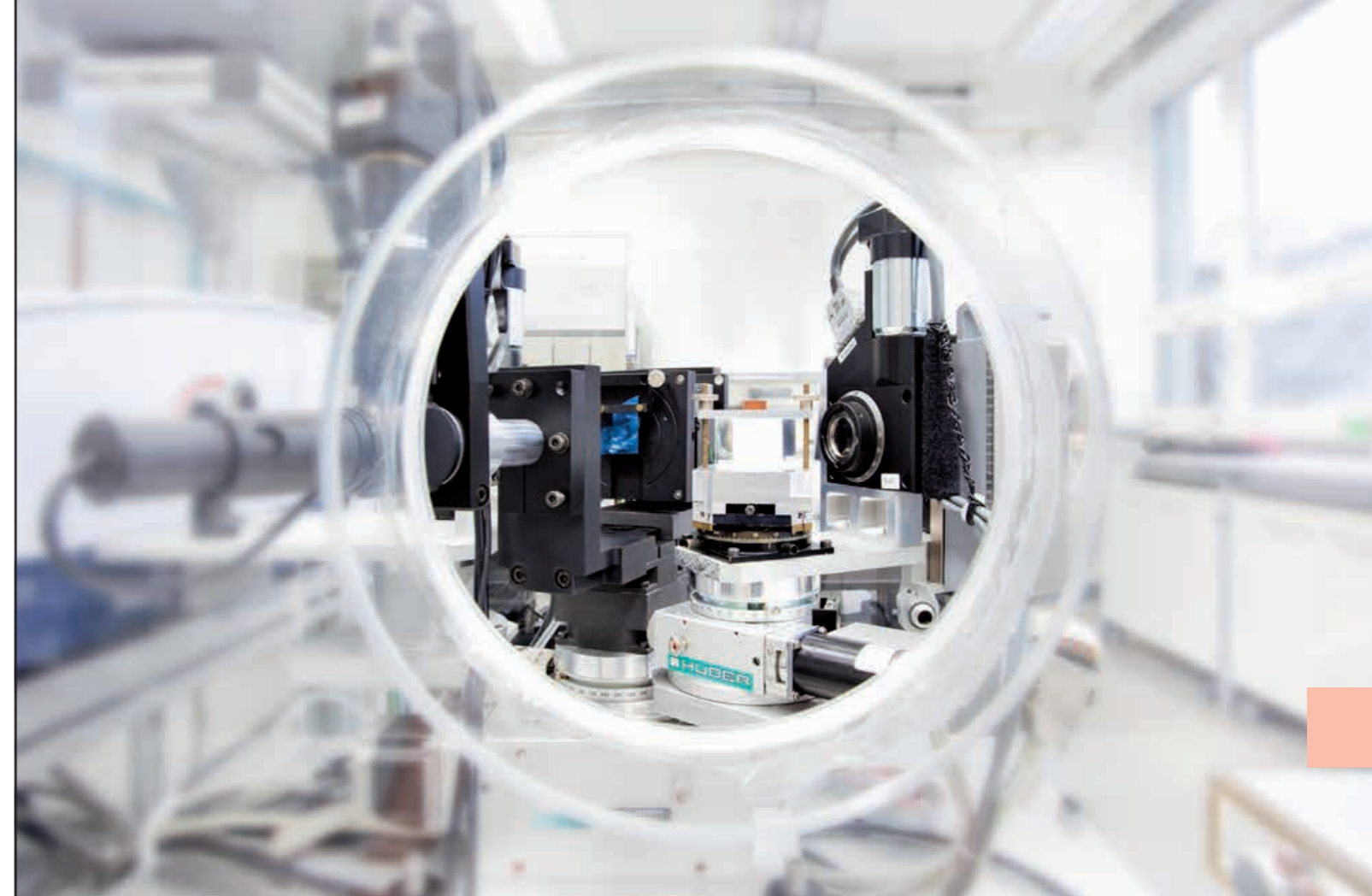
The infrared ellipsometer facilitates the contactless, non-destructive, label-free analysis of the structure and composition of sample materials.
